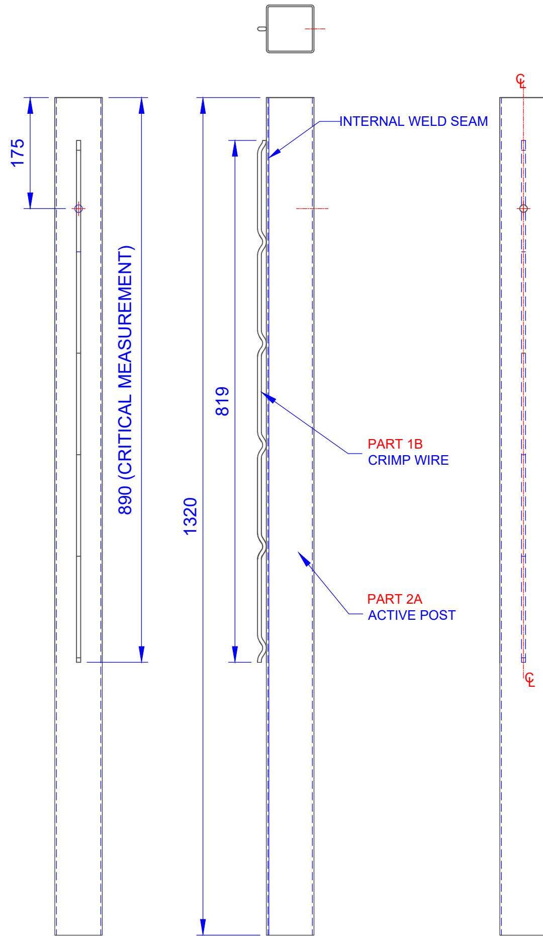
SUB ASSY 02 ACTIVE POST
