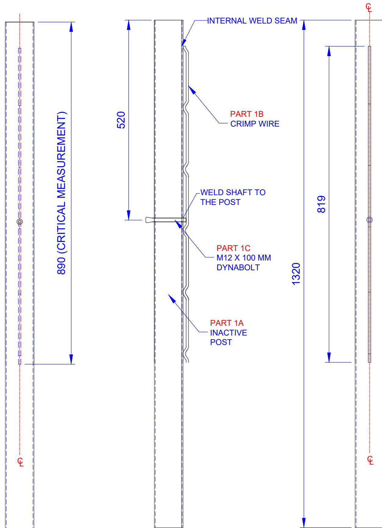
SUB ASSY 01 INACTIVE POST
