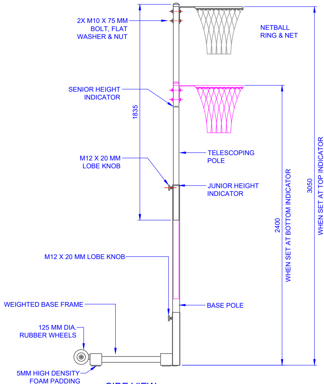
SIDE VIEW NSP60 PORTABLE NETBALL POST SCALE 1:20
