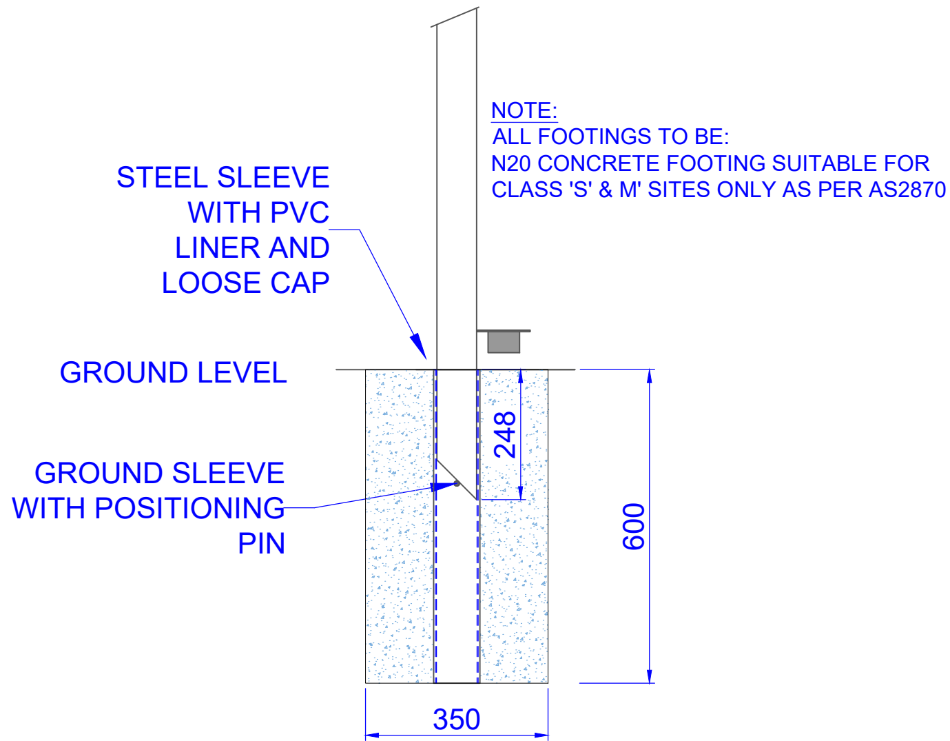
SLEEVE OPTION: ES76 PVC SLEEVE WITH EL76 LOOSE CAP
