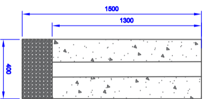
POLE FOOTING A (X3) FOR SOIL TYPES S, M
